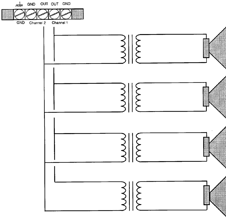
Fig. 1 70V Constant Voltage Distribution System
