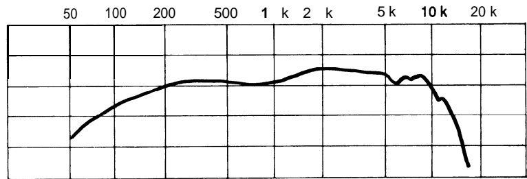
Figure 1. Frequency Response
