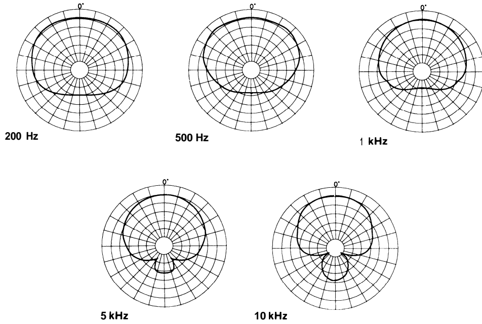
Figure 4. Polar Patterns
