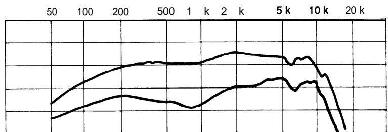
Figure 3. 0° and 180° Response
