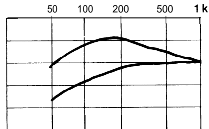
Figure 2. Proximity Effect
